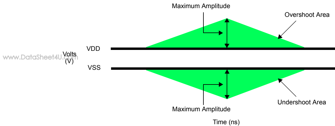
Figure 7. AC Overshoot and Undershoot Definition for Address and Control Pins
