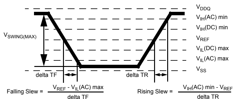
&lt; AC Input Test Signal Waveform &gt;
