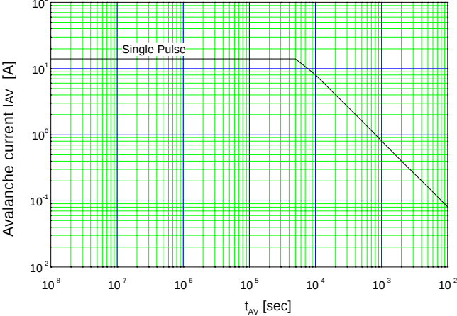
Maximum Avalanche Current Pulsewidth I_{AV}=f(t_{AV}) : starting T_{ch}=25^{\circ}C . V_{CC}=50V
