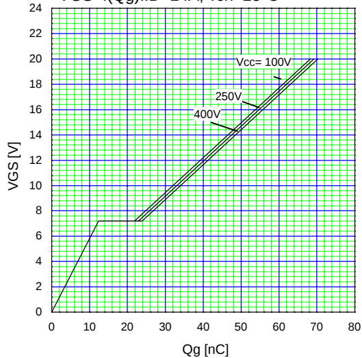
Typical Gate Charge Characteristics V_{GS} = f(Q_g): I_D = 14A, T_{ch} = 25^{\circ}C
