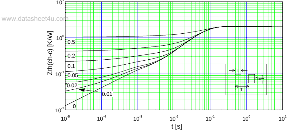
Transient Thermal impedance Z_{th(ch-c)}=f(t) parameter: D=t/T
