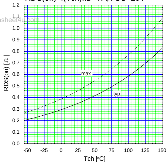
Drain-Source On-state Resistance R_{DS(on)} = f(T_{ch}): I_D = 7A, V_{GS} = 10V
