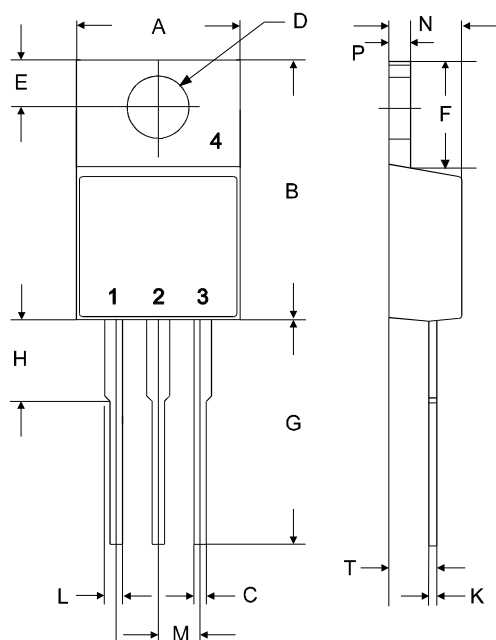
PG-TO220-3-1
