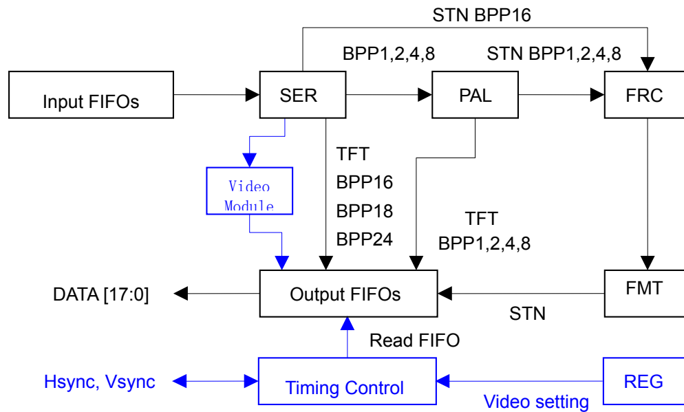
Figure 11-1 Block Diagram
