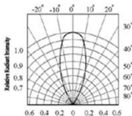
Radiation Diagram
