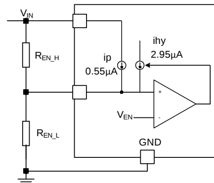
Figure 1. UVLO Setting
