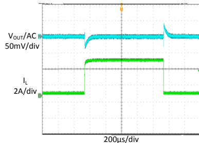
Load Transient
