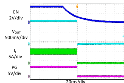
PG in Shutdown through Enable
