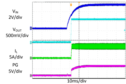
PG in Start-Up through VIN
