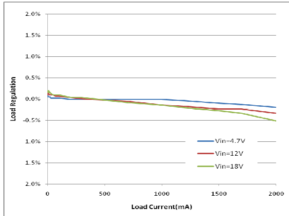
Figure 7. Output Voltage Regulation vs Load Current ( V_{out}=3.3V , L=3.3\mu H )
