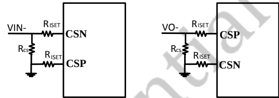
(a) Input current sense (b) output current sense
