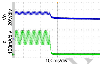
Power Off(Output)
