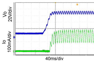
Start Up(Output)
