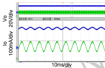
Steady State(Output)
