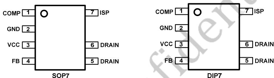
TOP VIEW
