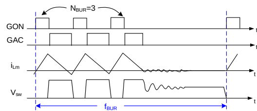
Figure 5: BUR Waveforms
