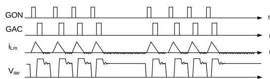
Figure 7: Burst Waveforms
