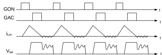
Figure 6: DCM Waveforms
