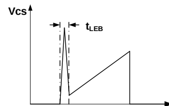
Figure 8: LEB Blanking
