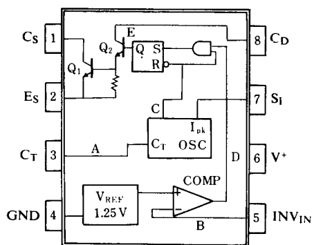
Fig. 1 Block Diagram
