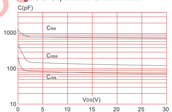
Figure 6: Capacitance Characteristics
