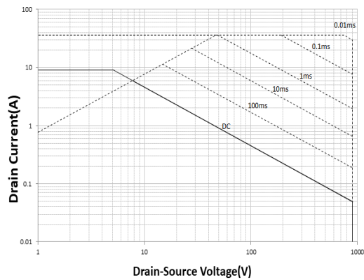
Maximum Safe Operating Area JCS9N90WT/ABT
