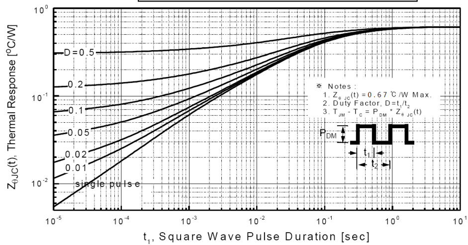
Transient Thermal Response Curve JCS9N90 WT/ABT
