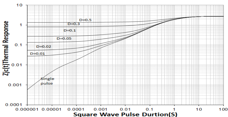
Transient Thermal Response Curve JCS9N90BT
