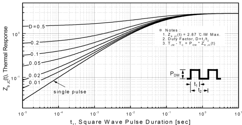
Transient Thermal Response Curve For JCS2N60C
