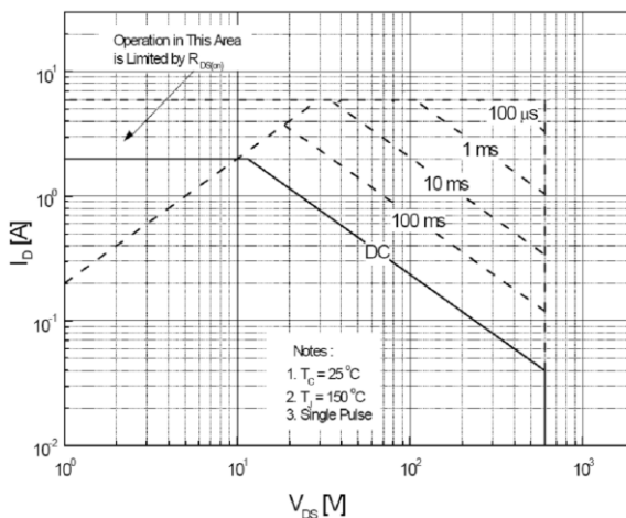
Maximum Safe Operating Area For JCS2N60F
