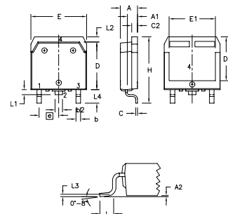
TO-268 Outline
