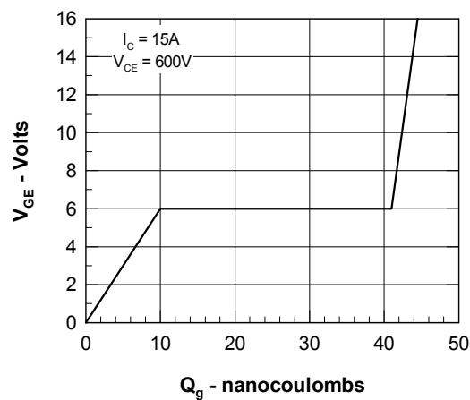
Fig. 9. Gate Charge
