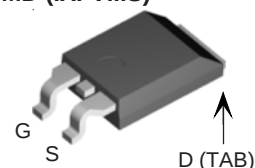
PLUS220SMD (IXFV...S)
