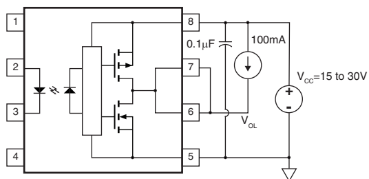
V_{OL} Test Circuit
