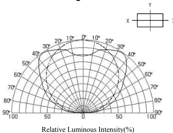
Radiation Diagram
