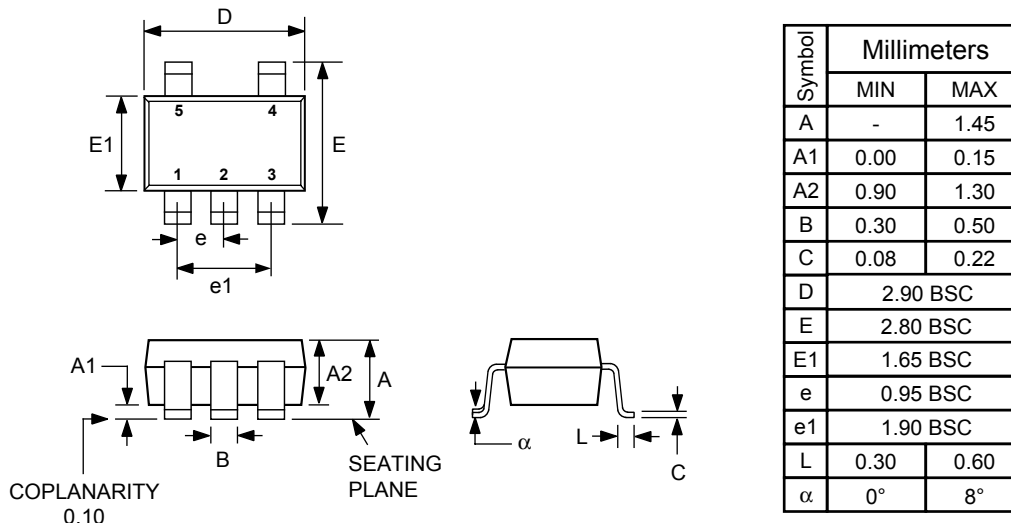
5-Lead Small Outline Transistor Package
