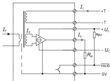
Figure 23: Standard characterization schematics for current output transducers
