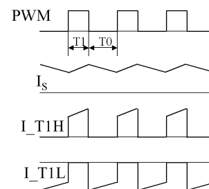
Figure 21: Current in transistors
