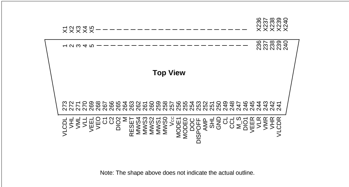
Figure 4-1. 273-pin TCP
