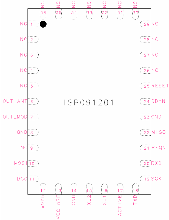
TOP VIEW
