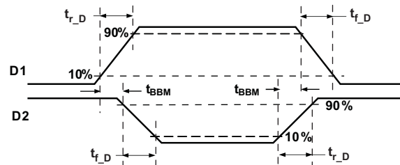
Figure 28. Transition Times and Break-Before-Make Time Delay for D1, D2 Outputs
