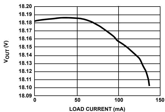
FIGURE 11. LOAD REGULATION ( V_{IN} = 3.6V )
