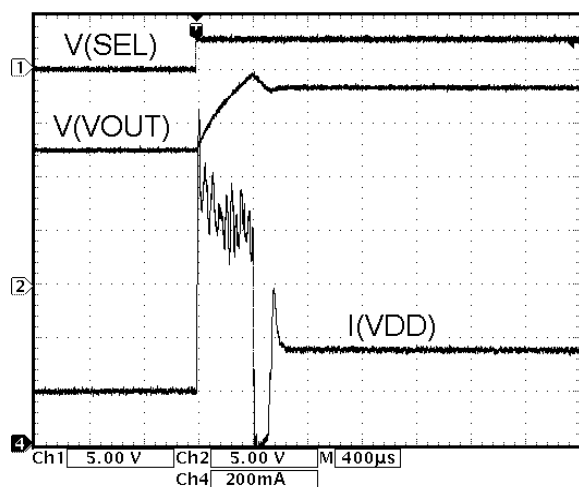
FIGURE 8. 12V->18V TRANSITION ( V_{DD} = 3.6V , R_L = 360\Omega )
