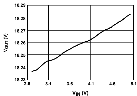
FIGURE 12. LINE REGULATION ( I_{OUT} = 30mA )
