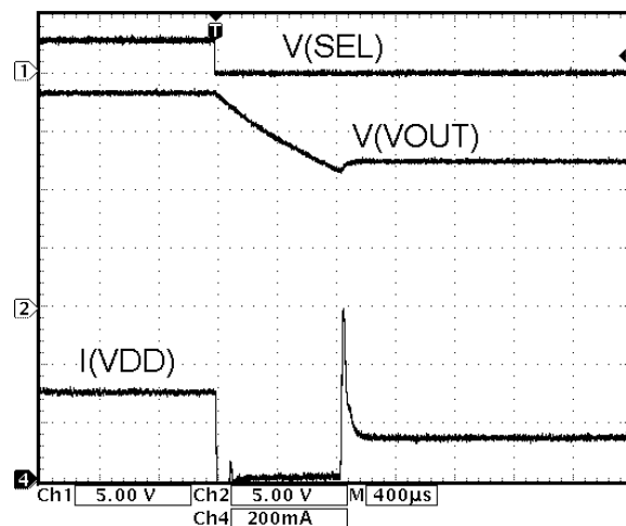
FIGURE 9. 18V->12V TRANSITION ( V_{DD} = 3.6V , R_L = 360\Omega )
