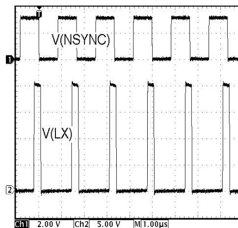
FIGURE 18. LX SYNCHRONIZATION WITH f(\text{SYNC}) = 600\text{kHz}
