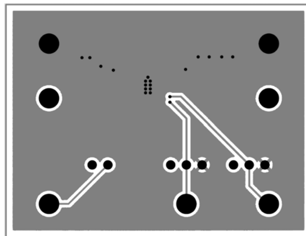
FIGURE 22. BOTTOM LAYER of the DEMO BOARD
