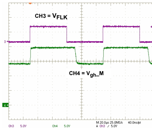
FIGURE 16. GPM WAVEFORM
