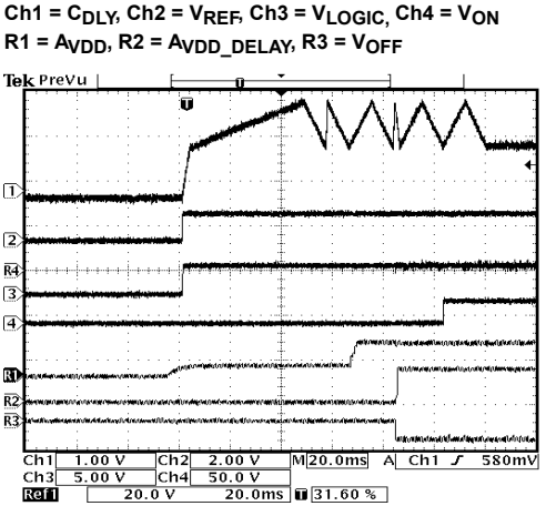
FIGURE 14. START-UP SEQUENCE
