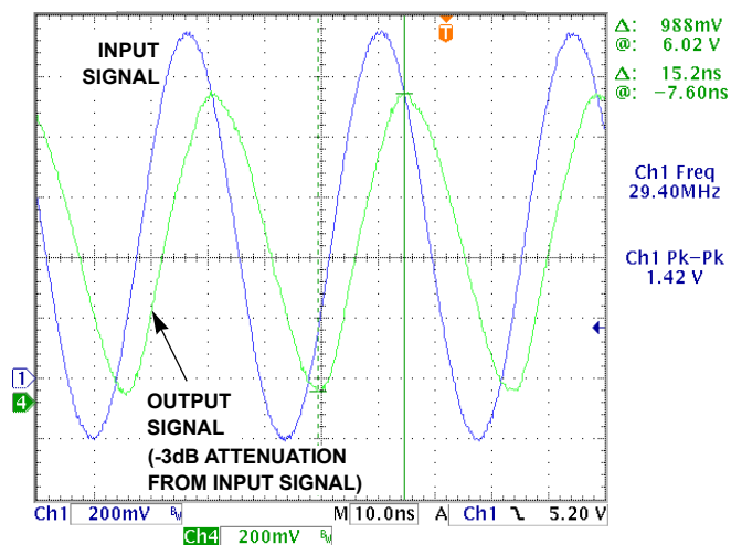
FIGURE 12. V_{COM} BANDWIDTH MEASUREMENT
