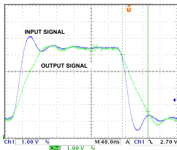
FIGURE 11. V_{COM} RISING SLEW RATE
