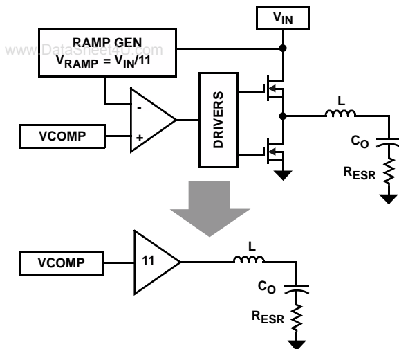
FIGURE 19. FOR SMALL SIGNAL AC ANALYSIS, THE PWM AND POWER STAGE CAN BE MODELED AS A SIMPLE GAIN OF 11
