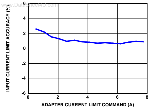
FIGURE 5. INPUT CURRENT LIMIT ACCURACY
