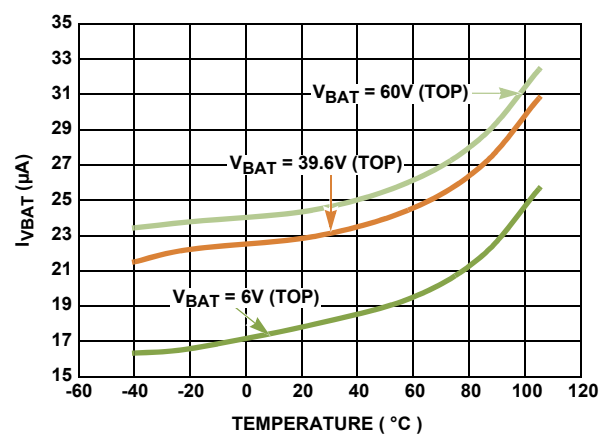
FIGURE 22C. PACK VOLTAGE SLEEP CURRENT vs TEMPERATURE AT 6V, 39.6V, 60V (DAISY CHAIN MODE)
