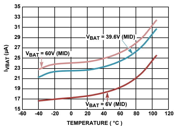
FIGURE 22D. PACK VOLTAGE SLEEP CURRENT vs TEMPERATURE AT 6V, 39.6V, 60V (DAISY CHAIN MODE)
