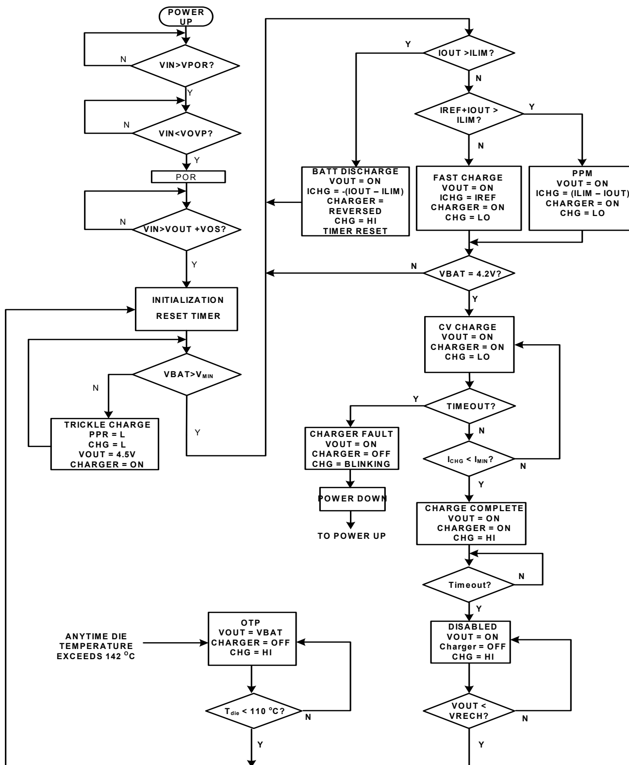
FIGURE 6. STATE DIAGRAM
