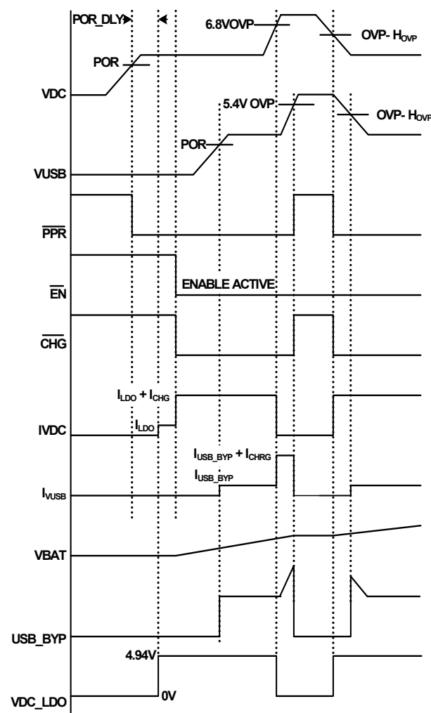
FIGURE 2. CHARGING PROFILE
