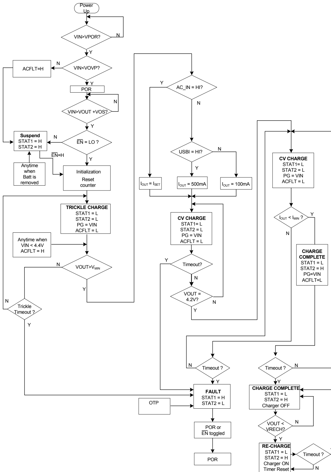
FIGURE 3. STATE DIAGRAM
