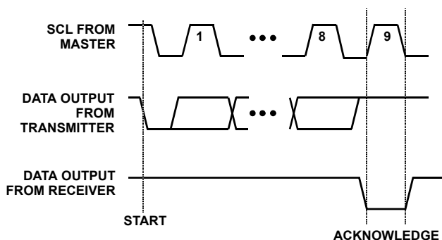
FIGURE 11. ACKNOWLEDGE RESPONSE FROM RECEIVER
