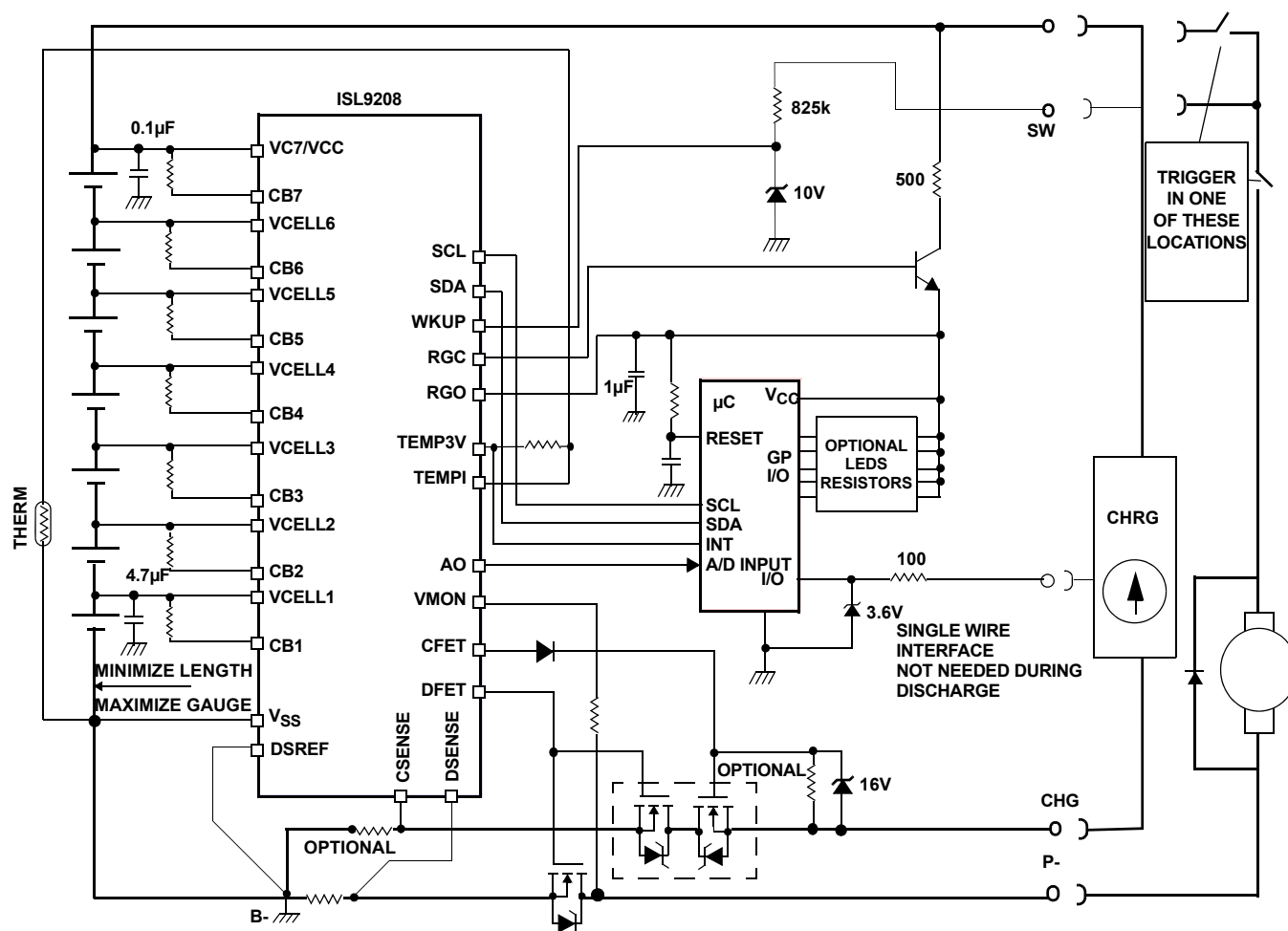
FIGURE 17. 7-CELL APPLICATION CIRCUIT WITH SWITCH WAKE-UP AND SEPARATE CHARGE/DISCHARGE
