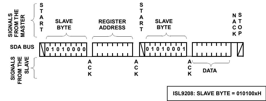
FIGURE 13. READ SEQUENCE
