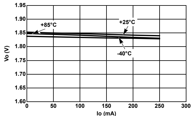
FIGURE 4. LOAD REGULATION vs TEMPERATURE ( V_{OUT} = 1.85V )
