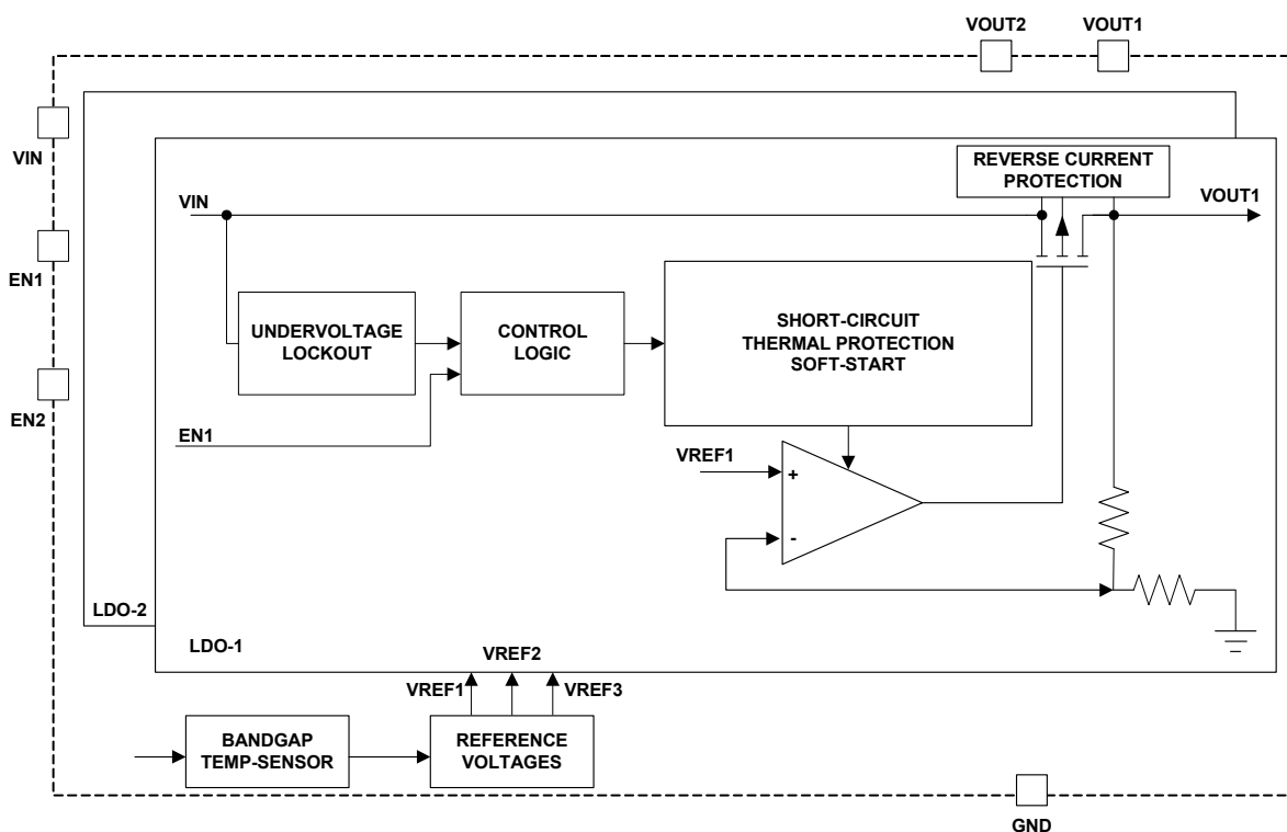
FIGURE 18. BLOCK DIAGRAM
