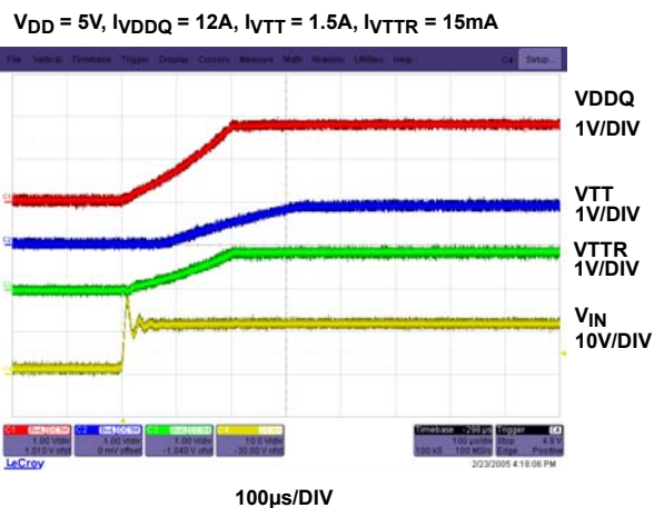
FIGURE 12. POWER-UP WAVEFORMS
