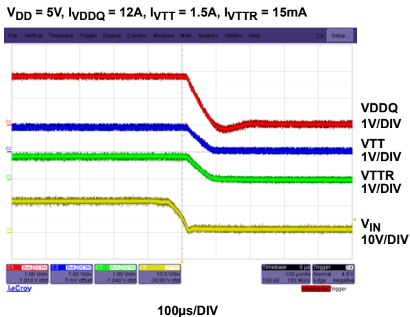
FIGURE 13. POWER-DOWN WAVEFORMS
