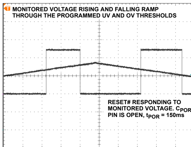
FIGURE 5. ISL88022EVAL1 3.3V UV AND OV DETECTION
