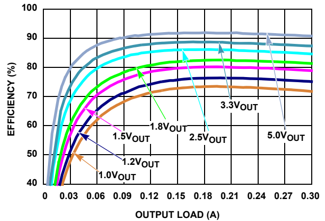
FIGURE 6. EFFICIENCY vs LOAD, PWM, V_{IN} = 12\text{V}
