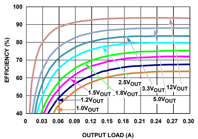
FIGURE 8. EFFICIENCY vs LOAD, PWM, V_{IN} = 24\text{V}
