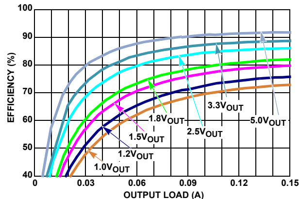
FIGURE 6. EFFICIENCY vs LOAD, PWM, V_{IN} = 12\text{V}
