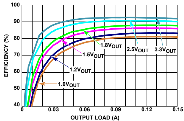
FIGURE 4. EFFICIENCY vs LOAD, PWM, V_{IN} = 5\text{V}
