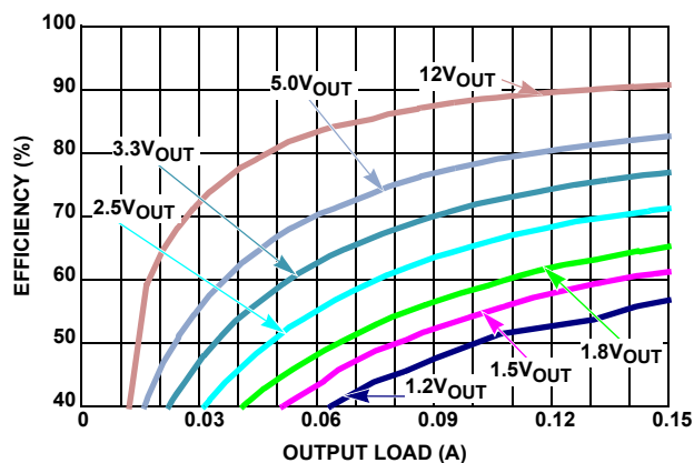
FIGURE 10. EFFICIENCY vs LOAD, PWM, V_{IN} = 36\text{V}
