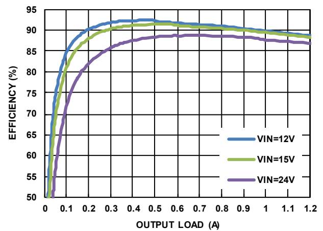
FIGURE 7. EFFICIENCY vs LOAD, PWM, V_{OUT} = 5\text{V} , L_1 = 22\mu\text{H}
