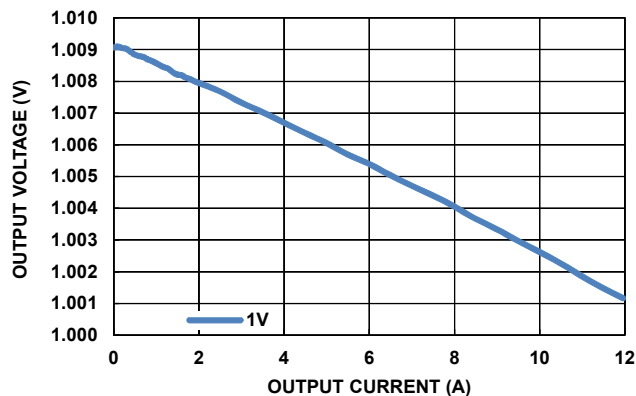
FIGURE 9. V_{OUT} REGULATION vs LOAD ( V_{IN} = 12V , CCM, 300kHz)
