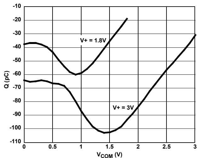
FIGURE 12. CHARGE INJECTION vs SWITCH VOLTAGE
