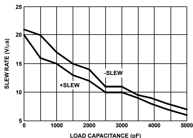
FIGURE 8. SLEW RATE vs LOAD CAPACITANCE
