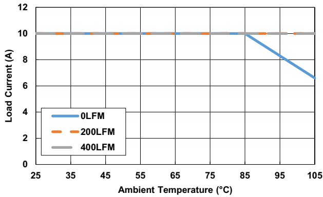
Figure 31. 0.6V OUT
