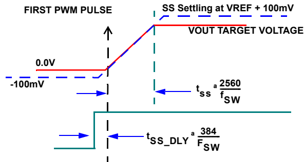
FIGURE 25. SOFT-START WITH V_{OUT} = 0V
