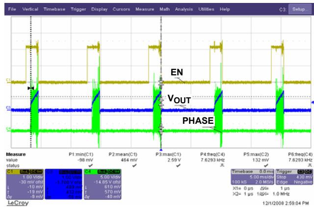
FIGURE 19. OVERCURRENT PROTECTION
