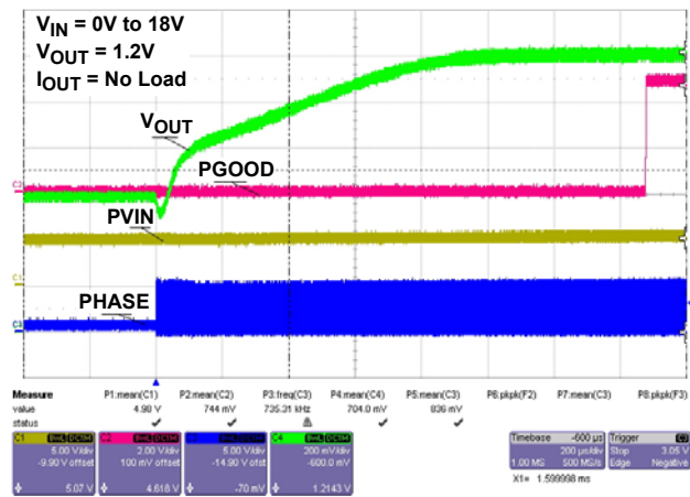
FIGURE 20. 50% PRE-BIAS START-UP
