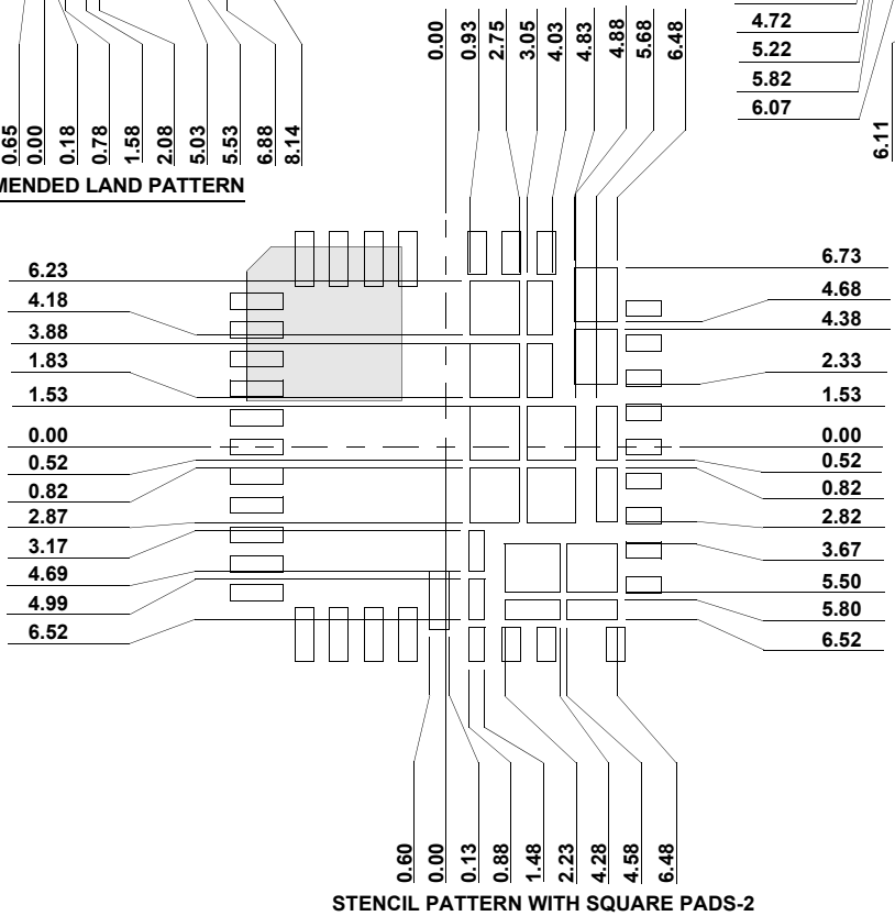
STENCIL PATTERN WITH SQUARE PADS-2
