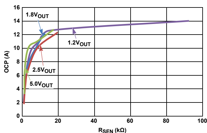
FIGURE 34. 20V IN
