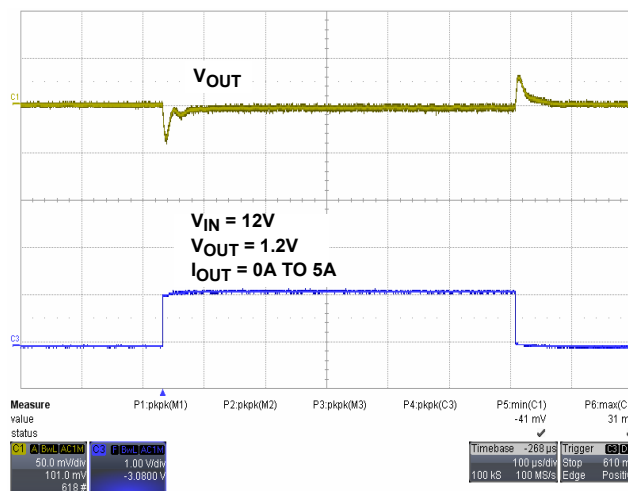
FIGURE 10. 1.2V TRANSIENT RESPONSE
