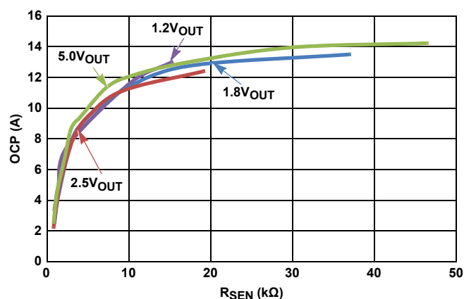
FIGURE 33. 12V IN
