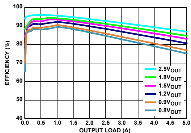
FIGURE 9. EFFICIENCY vs LOAD (2MHz 3.3V V_{IN} PFM)
