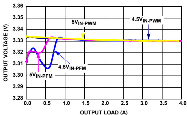
FIGURE 12. V_{OUT} REGULATION vs LOAD (1MHz, V_{OUT} = 3.3\text{V} )
