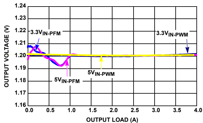
FIGURE 8. V_{OUT} REGULATION vs LOAD (1MHz, V_{OUT} = 1.2\text{V} )
