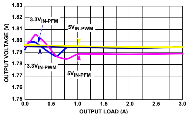
FIGURE 10. V_{OUT} REGULATION vs LOAD (1MHz, V_{OUT} = 1.8\text{V} )
