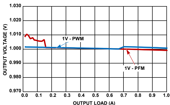
FIGURE 4. VOUT REGULATION vs LOAD ( 3.3V_{IN} , T_A = +25^\circ\text{C} )
