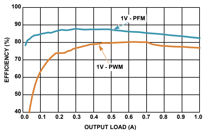
FIGURE 2. EFFICIENCY vs LOAD ( 3.3V_{IN} , T_A = +25^\circ\text{C} )
