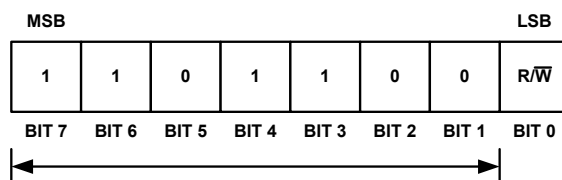
FIGURE 37. I 2 C SLAVE ADDRESS
