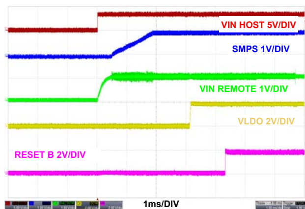
FIGURE 6. START-UP WITH VIN HOST = 3.3V AT NO LOAD (PFM)
