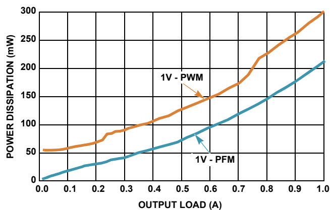
FIGURE 3. POWER DISSIPATION vs LOAD ( 3.3V_{IN} , T_A = +25^\circ\text{C} )
