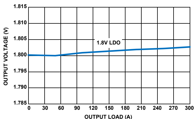
FIGURE 5. VOUT REGULATION vs LOAD ( 3.3V_{IN} , T_A = +25^\circ\text{C} )
